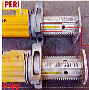
The measuring tape inside the PERI MULTIPROP has 'PERI' on it. There is one rivet at each end of the tape, whereas the counterfeit version has rivets along its entire length.
