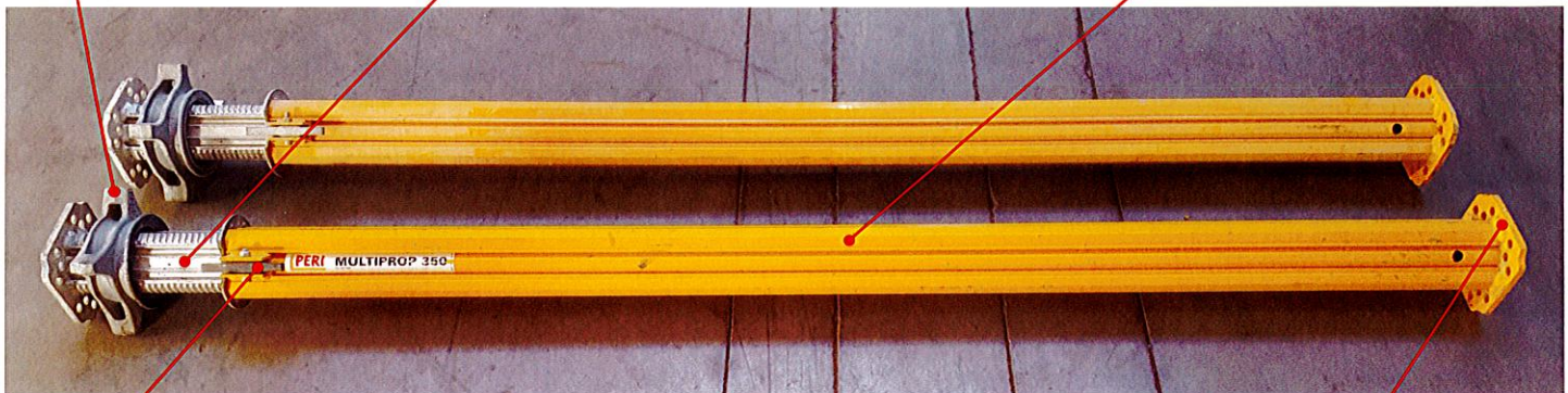
Props side-by-side; PERI MULTIPROP (bottom) and counterfeit version (top).
